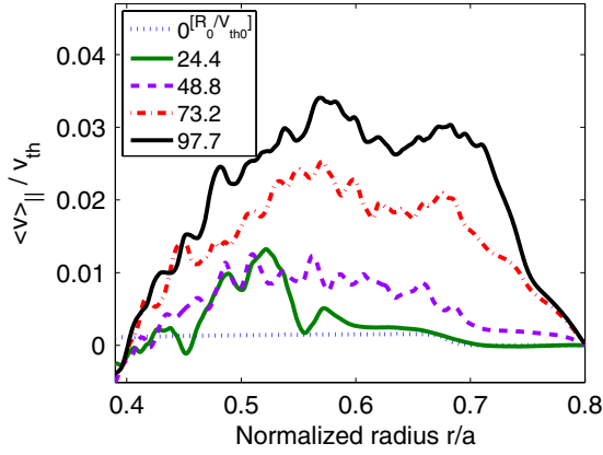
Figure 4. Parallel flow develops in GYSELA without torque at t = 0, 24.4, 48.8, 73.2 and 97.7 R_0/v_{th} . 110 R_0/v_{th} is corresponding to 1 ms.
