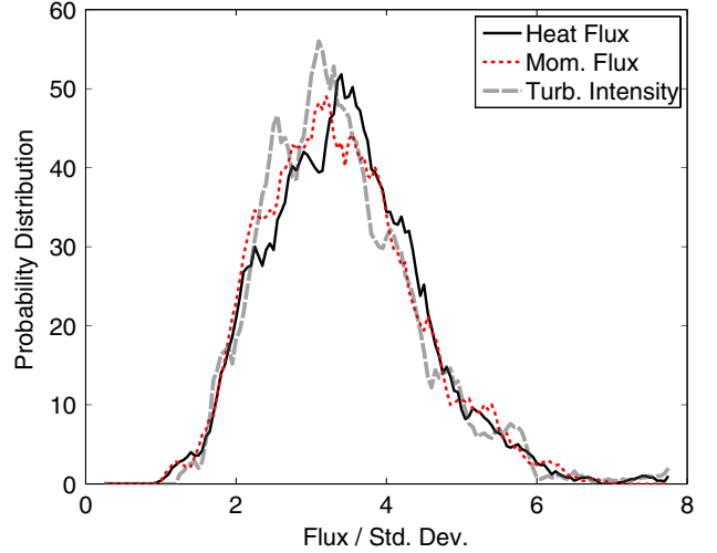
Figure 7. Probability distribution function of outward heat flux (solid), the negative of the momentum flux (dotted), and turbulence intensity (dashed) at r/a = 0.76 in XGC1p simulation with R/L_T \approx 6 . The x -axis is normalized in the standard deviation. The two distribution functions are similar, including mean value. Note that, for cancellation simulations, the non-zero mean momentum flux, which gives co-current rotation, is cancelled by external torque so as to keep the plasma stationary.
